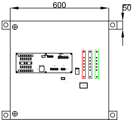
INTERNAL VIEW
